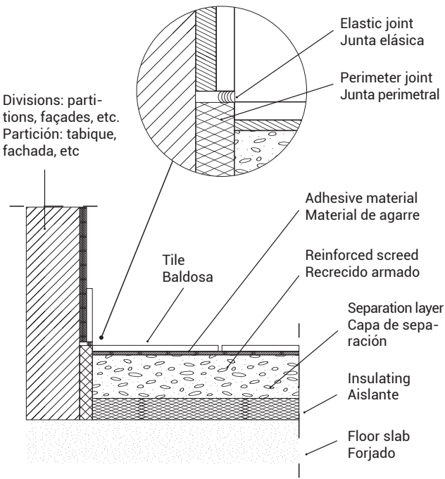
Detail of perimeter joint with sealant | Detalle de junta perimetral con sellante (UNE 138002:2017)
